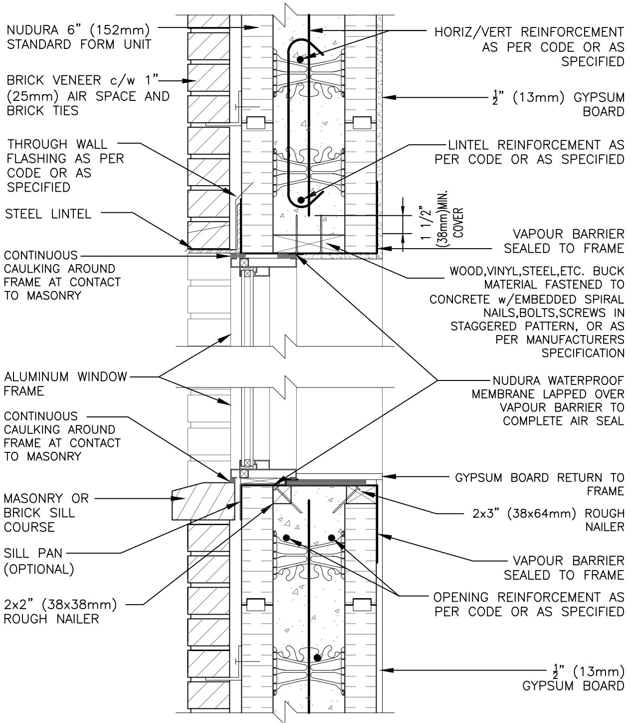
THIS DETAIL IS SUITABLE FOR NON-COMBUSTIBLE 1 TO 3 STOREY HIGH APPLICATIONS AS PERMITTED UNDER LOCAL CODES; FOR WINDOWS IN BRICK CLAD MULTI-STOREY APPLICATIONS, REFER TO DETAIL E6D03 UNDER THIS SECTION
