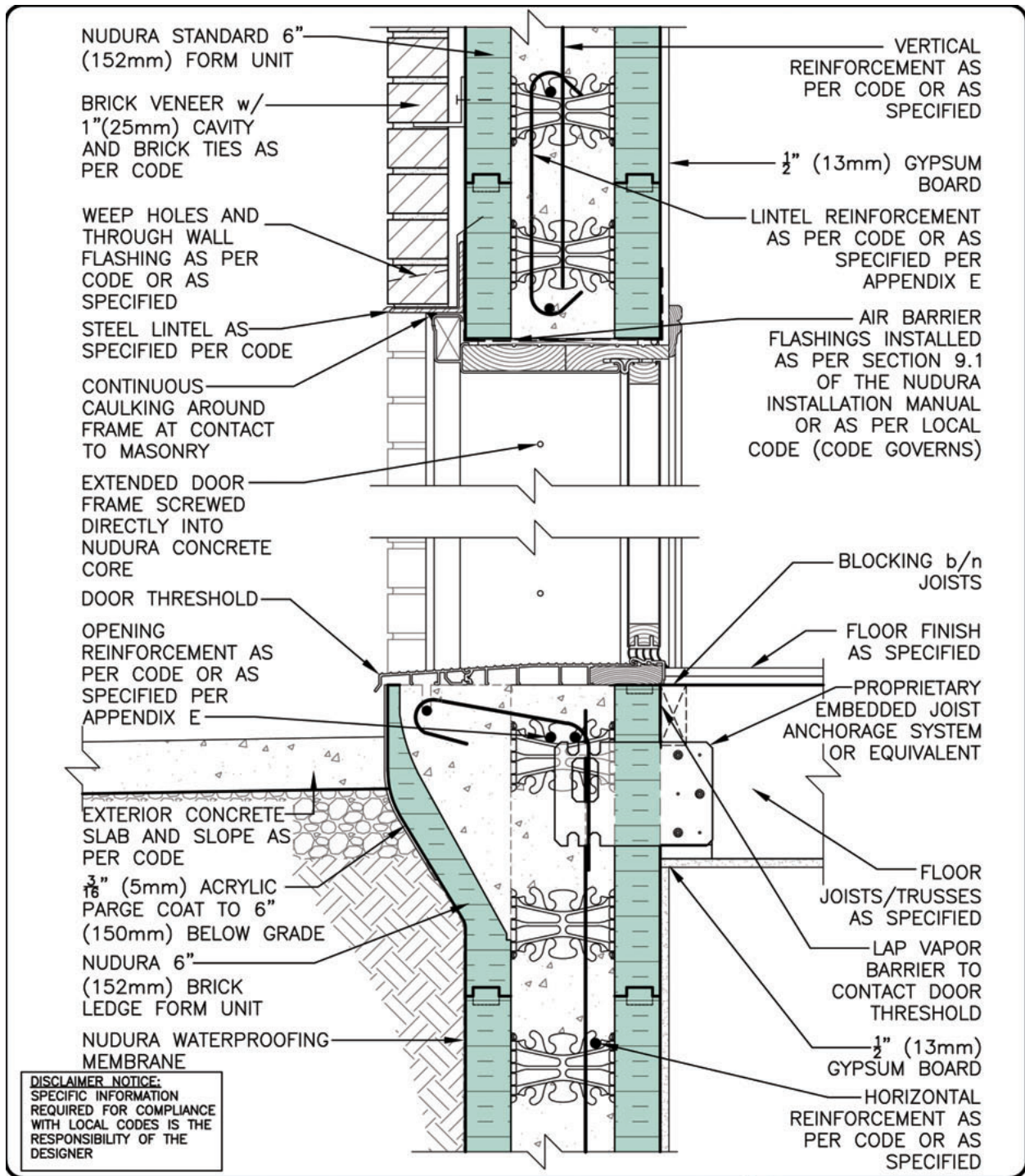
STANDARD 6" FORM UNIT DOOR HEAD/THRESHOLD DETAIL BRICK VENEER FINISH
