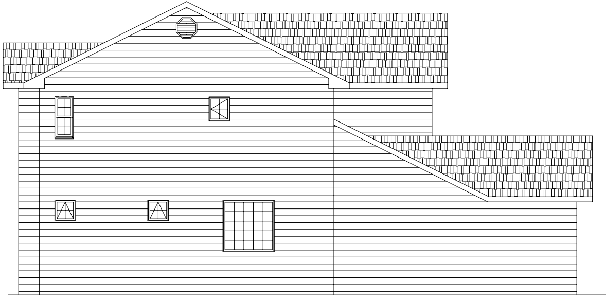
Figure 7 Left elevation.
