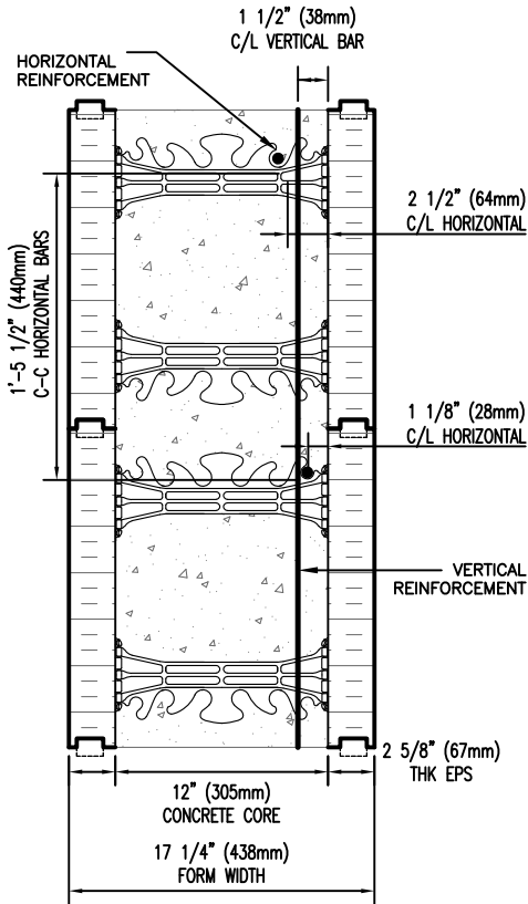
VERTICAL BARS OFF CENTER TYPICAL BELOW GRADE
