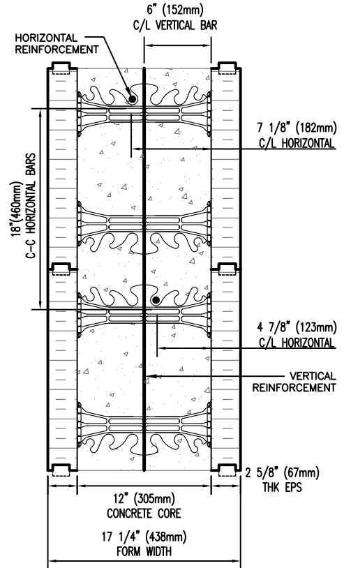
VERTICAL BARS AT CENTER TYPICAL ABOVE GRADE
